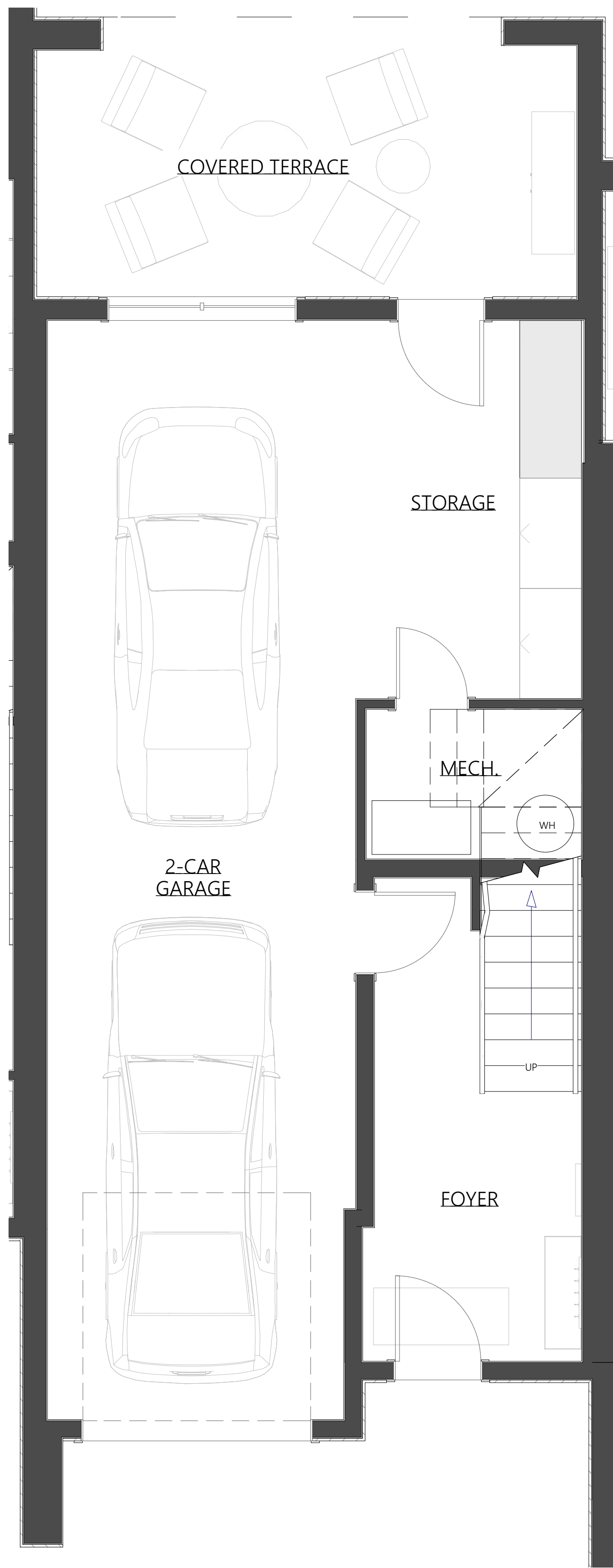
GROUND FLOOR
