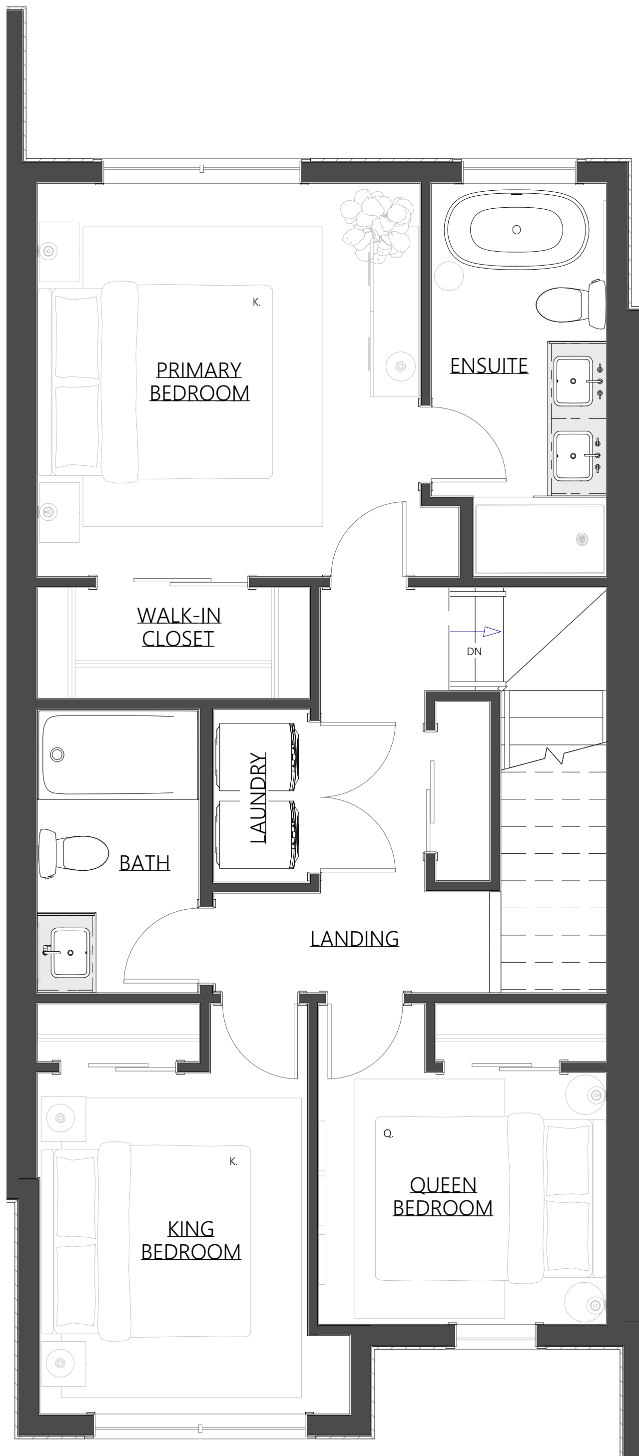
THIRD FLOOR
