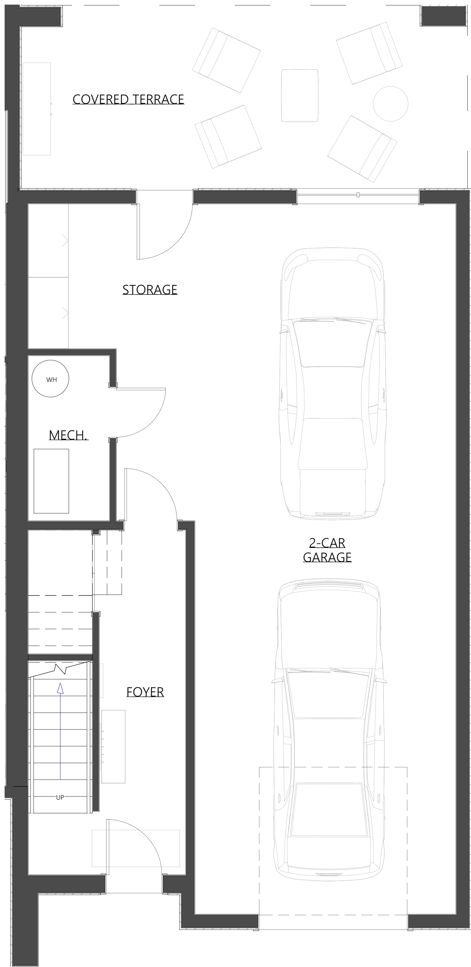
GROUND FLOOR
