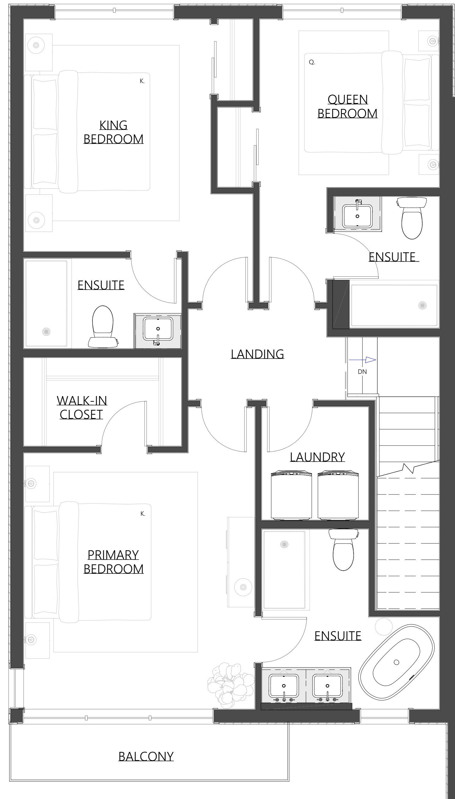
THIRD FLOOR
