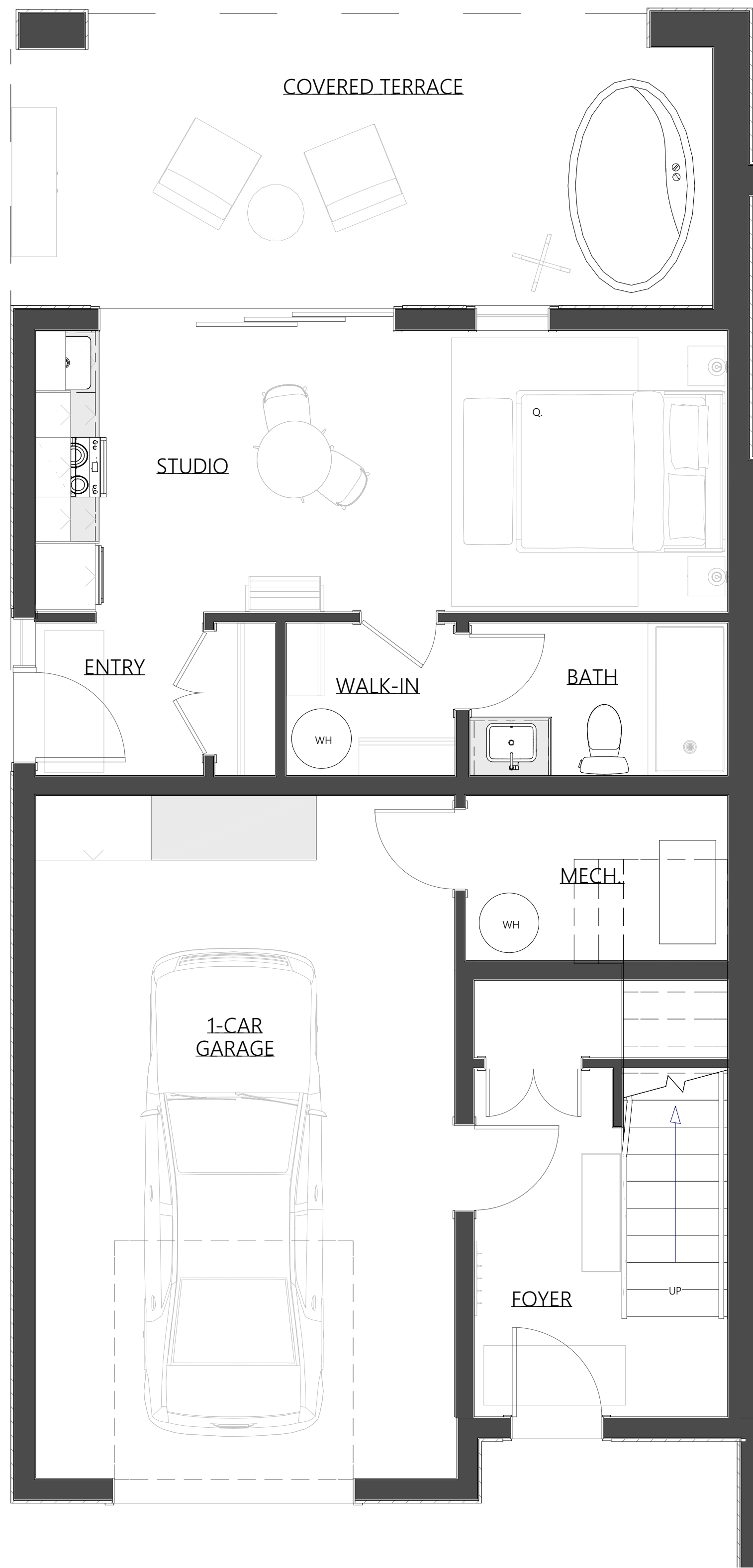
GROUND FLOOR
