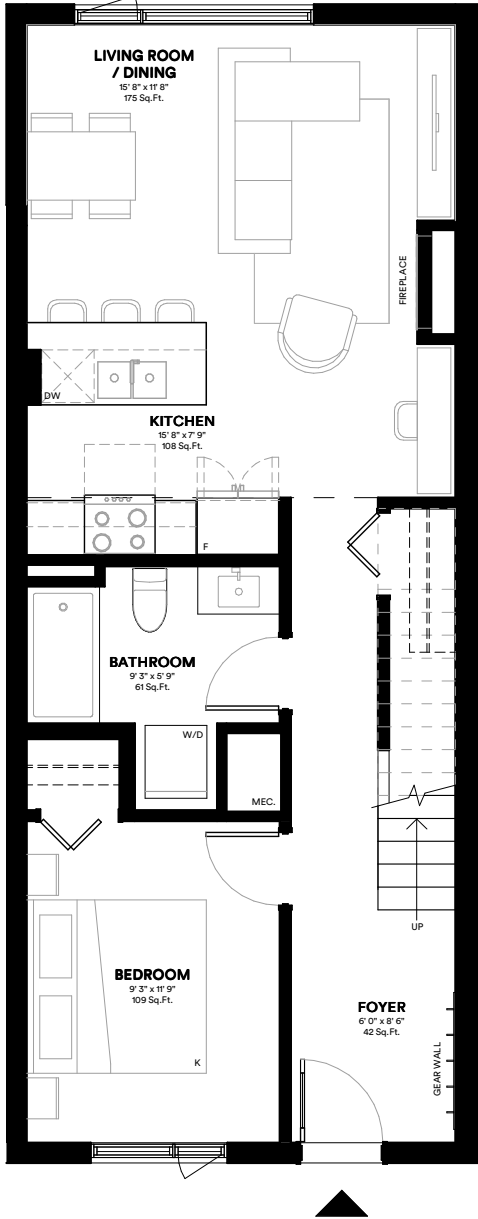
LEVEL 3 | 640 Sq.Ft.
