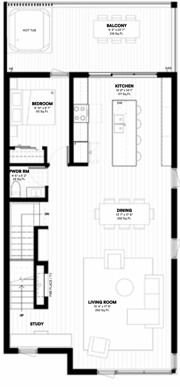
SECOND FLOOR 880 SQ FT
