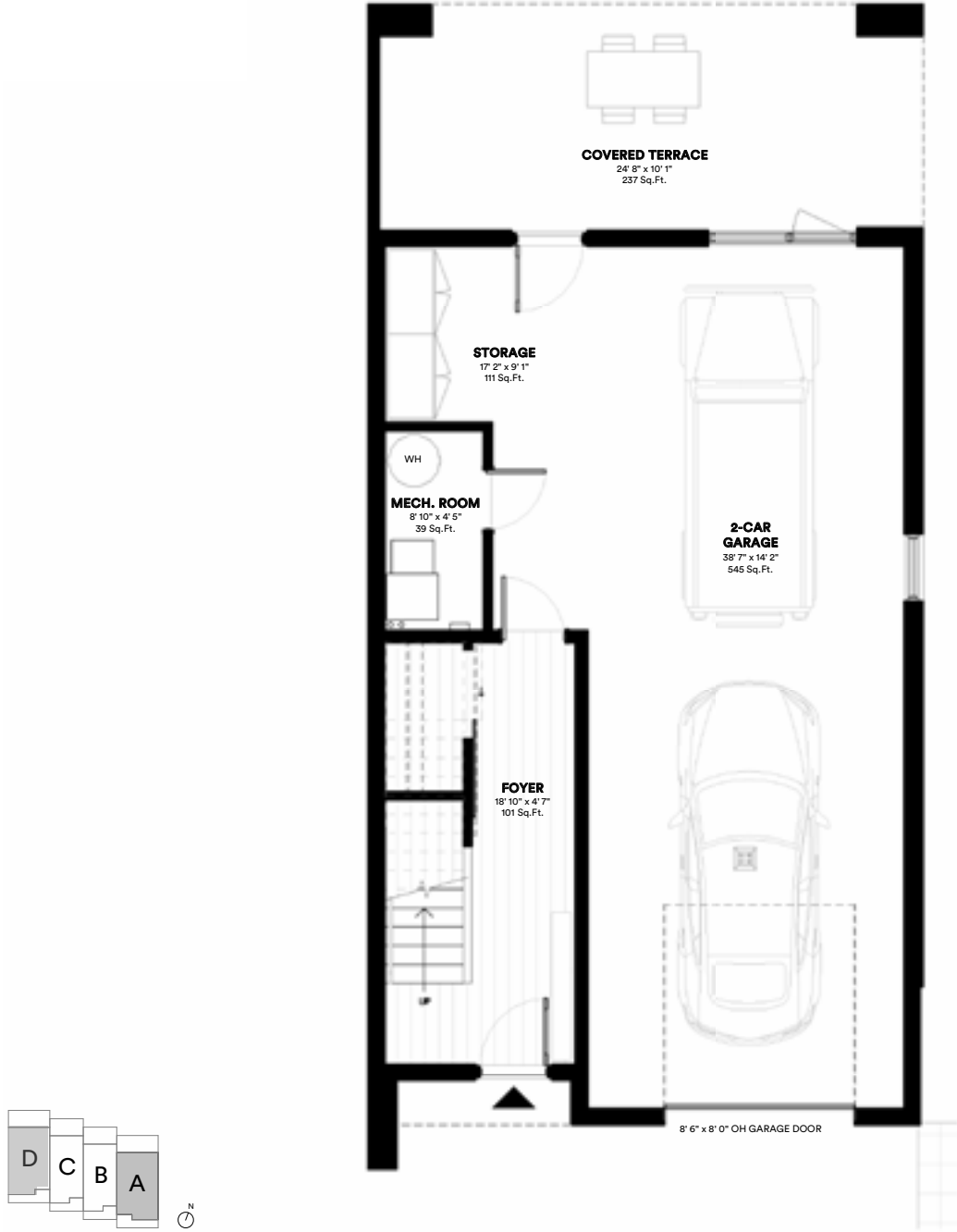
GROUND FLOOR 876 SQ FT
