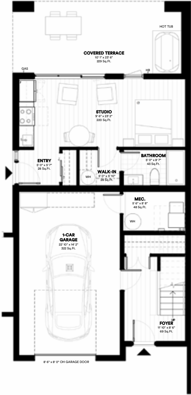
GROUND FLOOR 876 SQ FT Incl. Studio | 354 SQ FT
