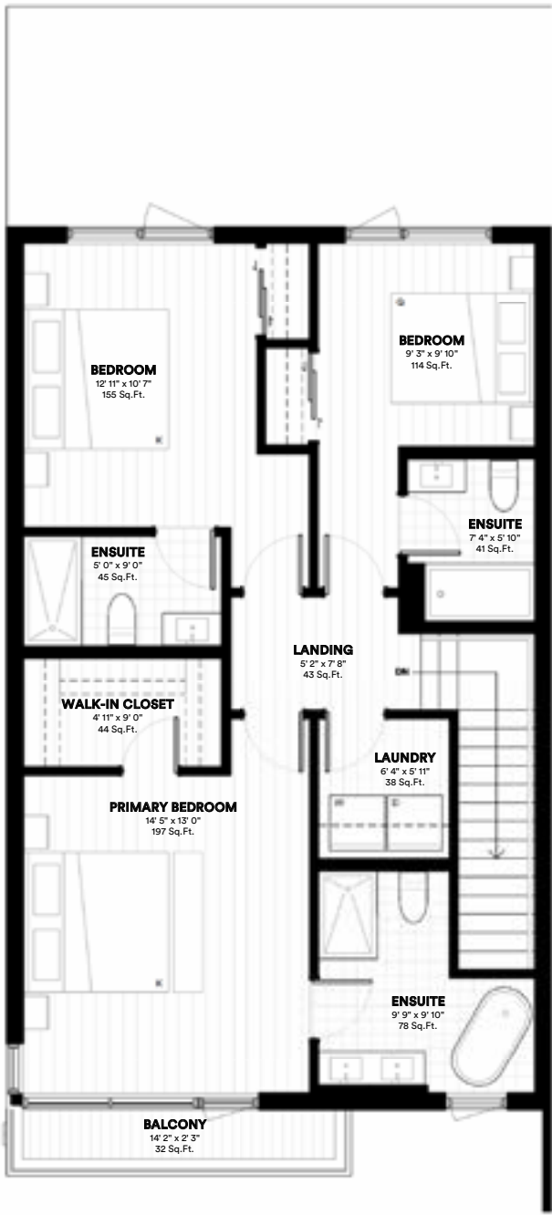
THIRD FLOOR 835 SQ FT
