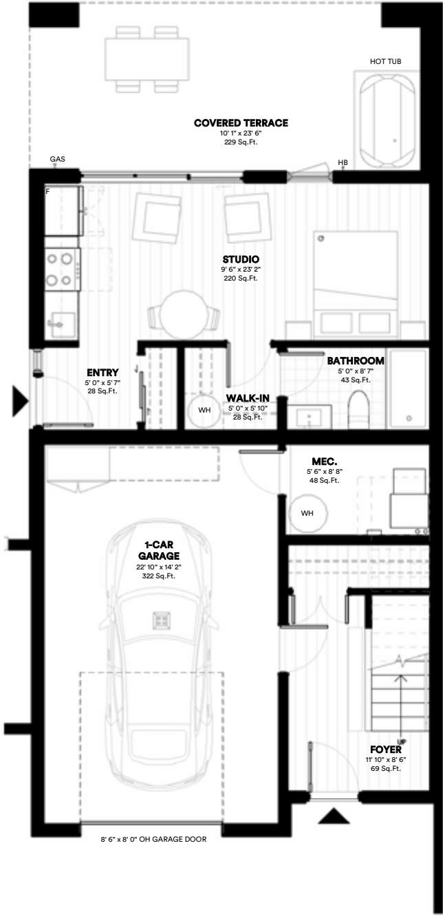
GROUND FLOOR
