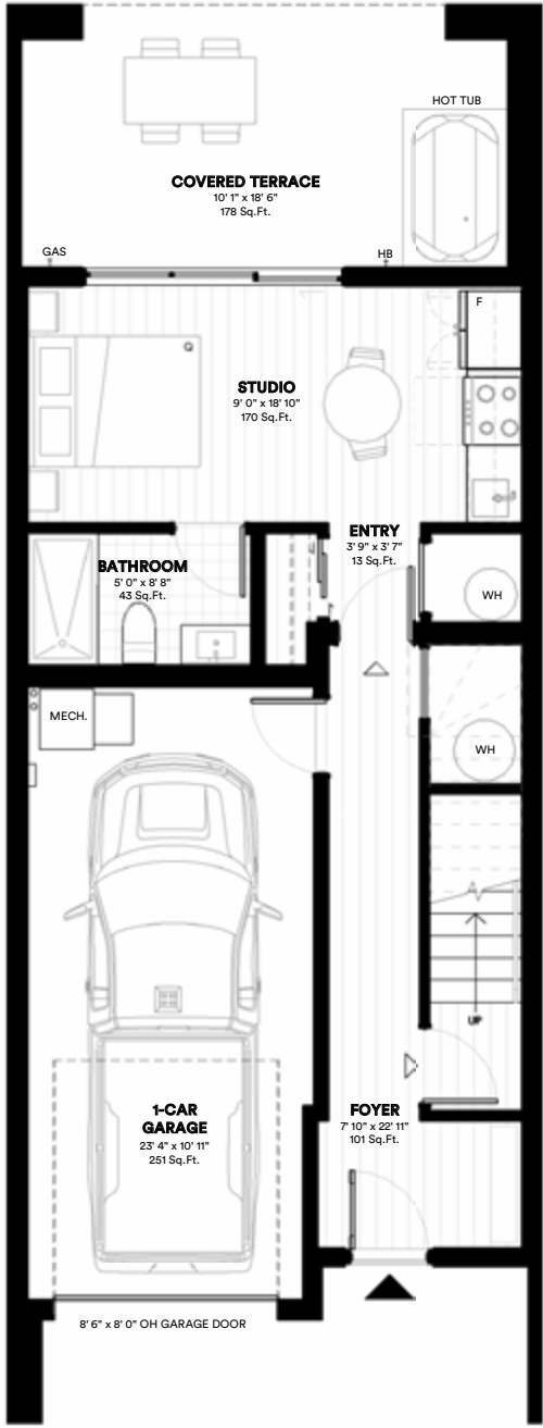
GROUND FLOOR 709 SQ FT Incl. Studio | 267 SQ FT
