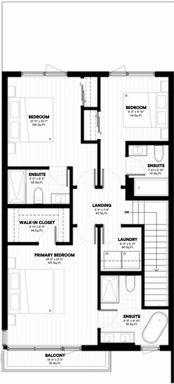
THIRD FLOOR
