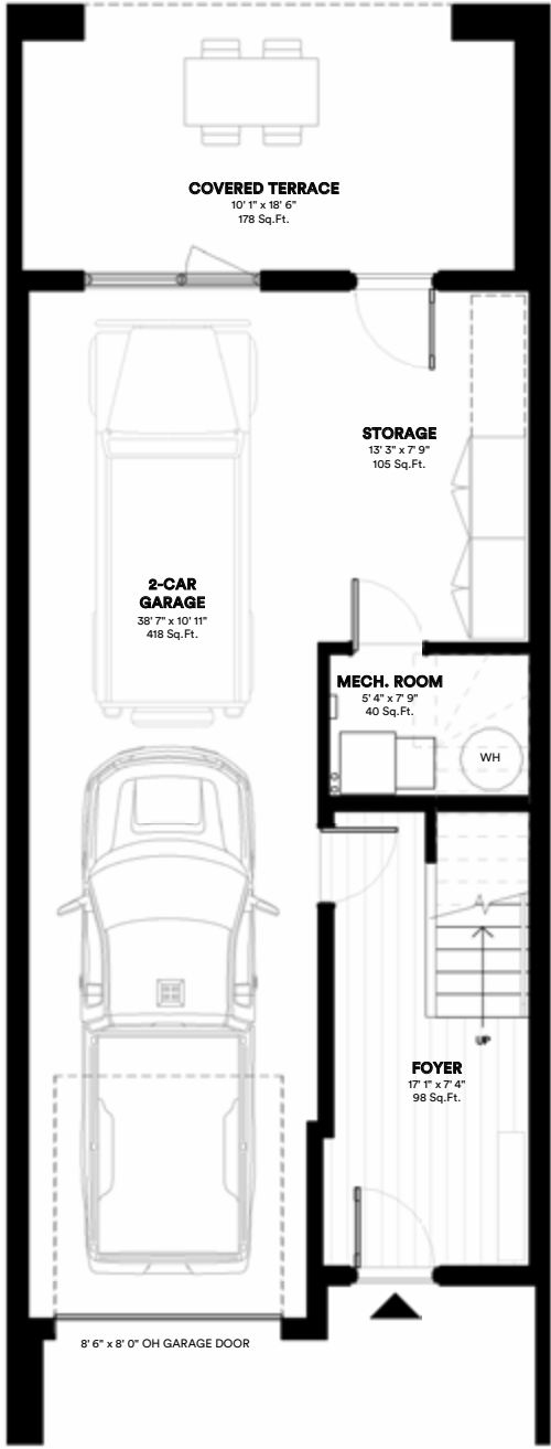
GROUND FLOOR 709 SQ FT
